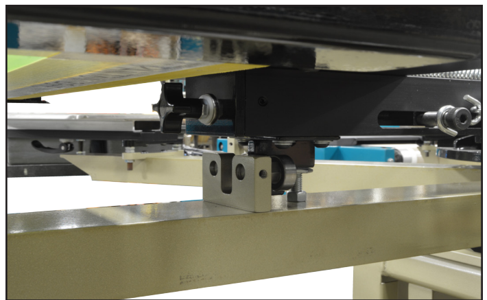
Heavy-duty lock-in print head facilitates precise multicolor printing.
