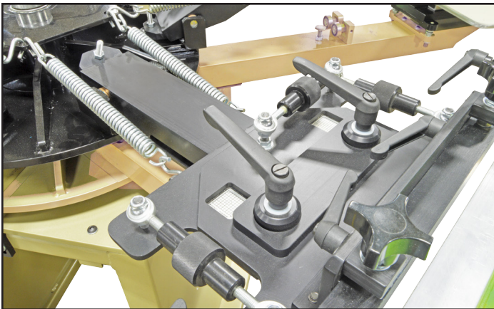
Precision multi-directional micro-registration for outstanding accuracy and control.
