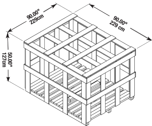
The original Rototex crate size.
